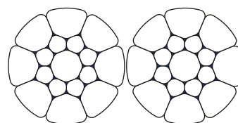
compacted strand
